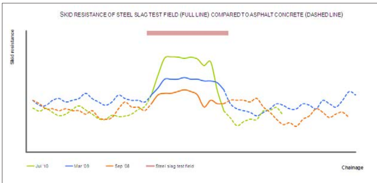
Figure 1: Development of the skid resistance of an EAF C steel slag aggregate wearing course
