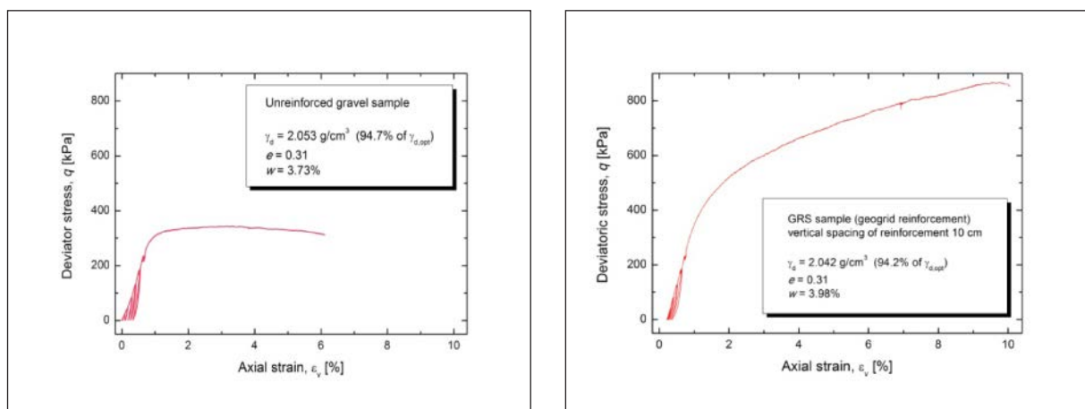
Fig. 1: Drained triaxial compression test with (a) unreinforced and (b) reinforced granular sample
