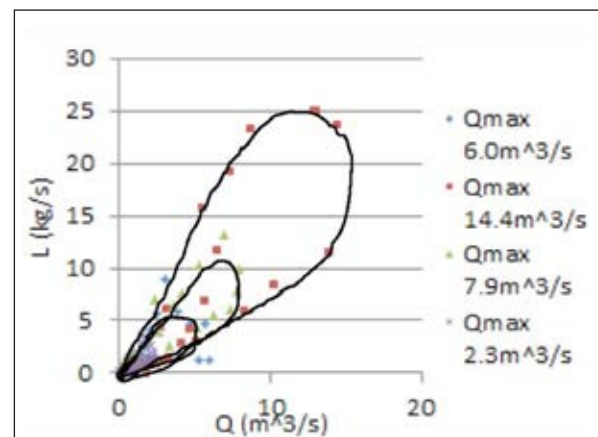
Fig.9 L-Q curve at the upstream point No.4
