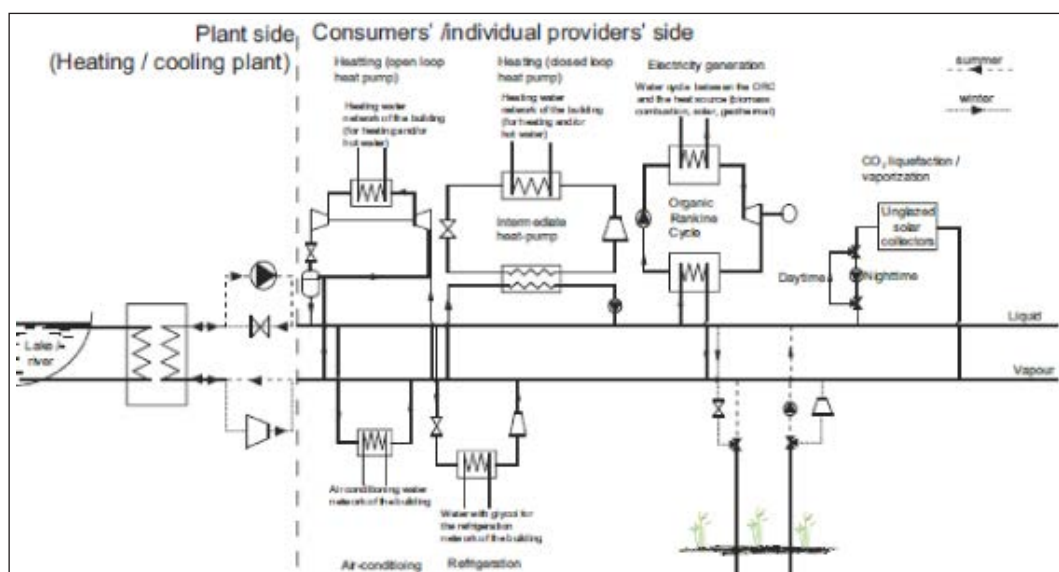
Figure 5: District heating and cooling network based on the distribution of \text{CO}_2 [10]
