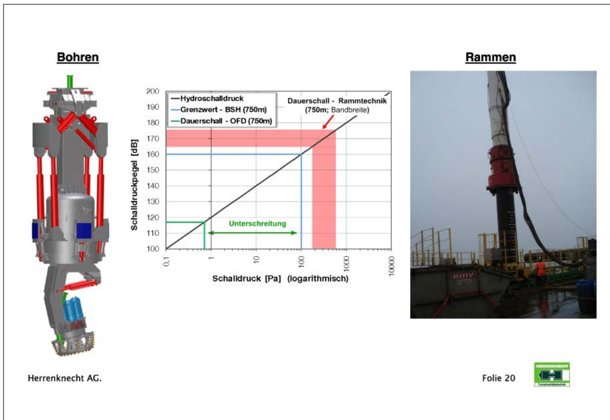
Fig. 17: Sound level measures OFD (green) – BSH-value (blue) – piling (red)
