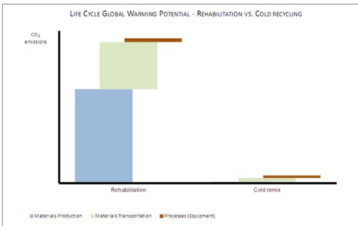
Figure 3: Global warming potential in the case of the investigated asphalt and unbound layers
