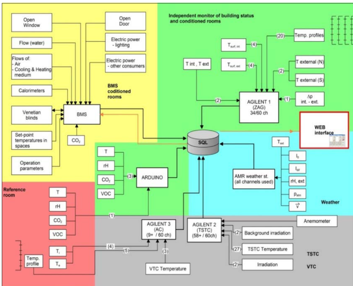
Illustration 4. General scheme of the monitoring system.
