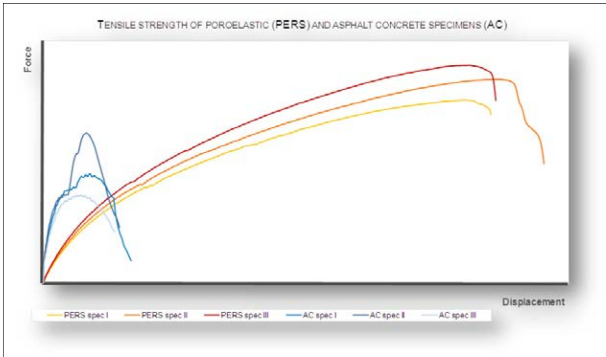
Figure 2: The measured tensile strengths of test specimens made of poroelastic and asphalt concrete
