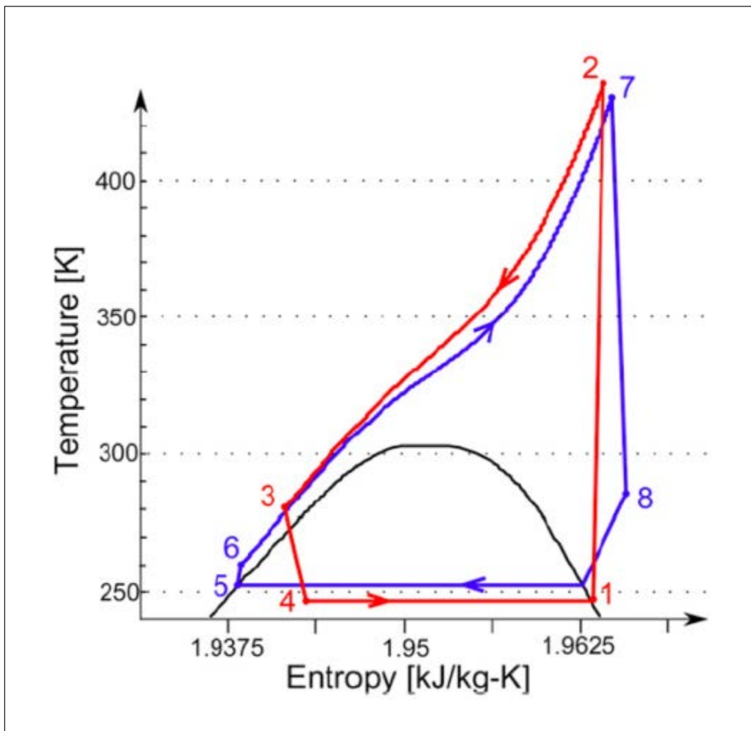
Figure 6: Alternate heat pump and power CO 2 cycles for electricity storage via a hot water storage tank [13]
