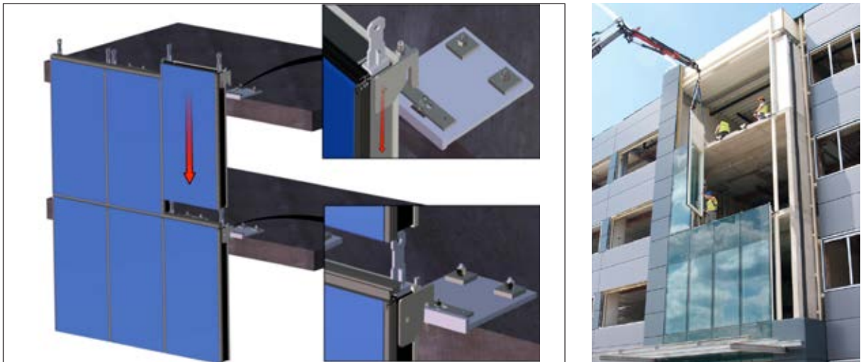
Fig 3: Installation of Qbiss Air elements
