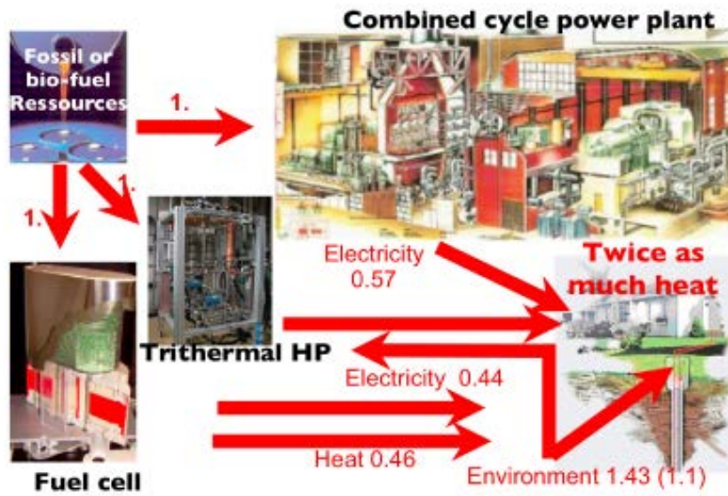
Figure 2: Examples of technological combinations to supply heat more ecoefficiently than with boilers
