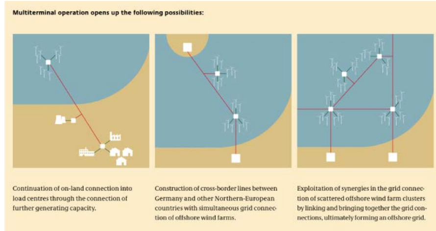
Fig. 5: Connection of wind farms to the land grid
