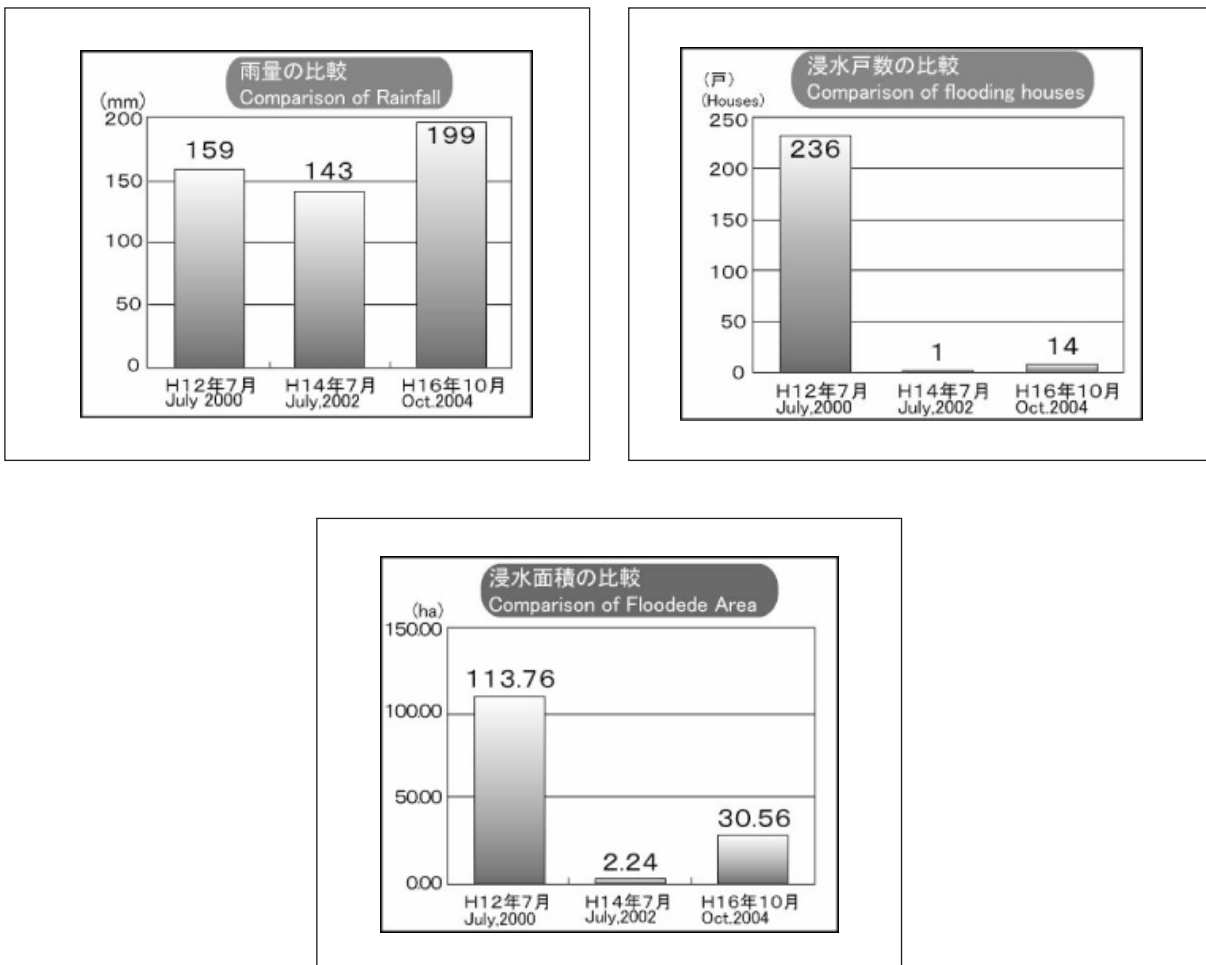
Figure12. Comparison of Rainfall, Flooding Houses, Flooding Area
