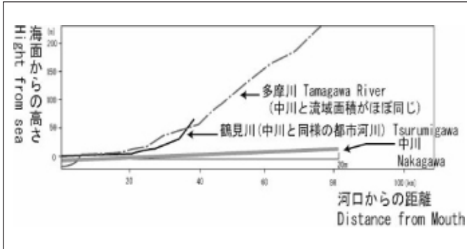
Figure 7 Bed Slope
