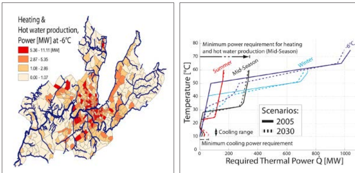
Figure 4: Heating needs of the canton of Geneva and composites of the demand [9]
