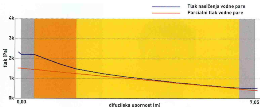
Graf 1: Porobeton + EPS + 'ZSPVDU'
